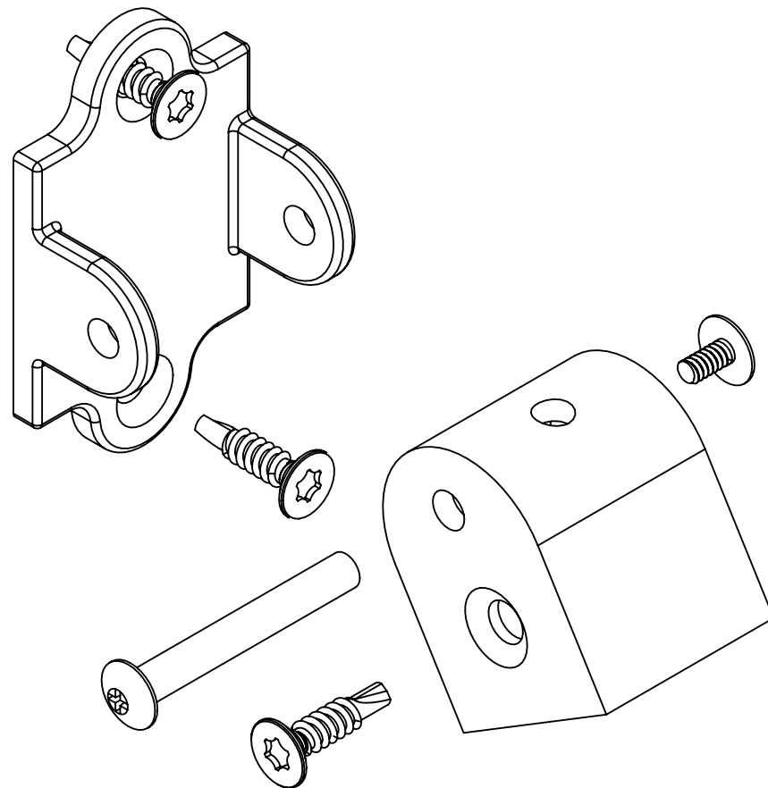
25mm Superior Stair Bracket Supplied With Fixings & Used With Raked Panel 64ARP10B
