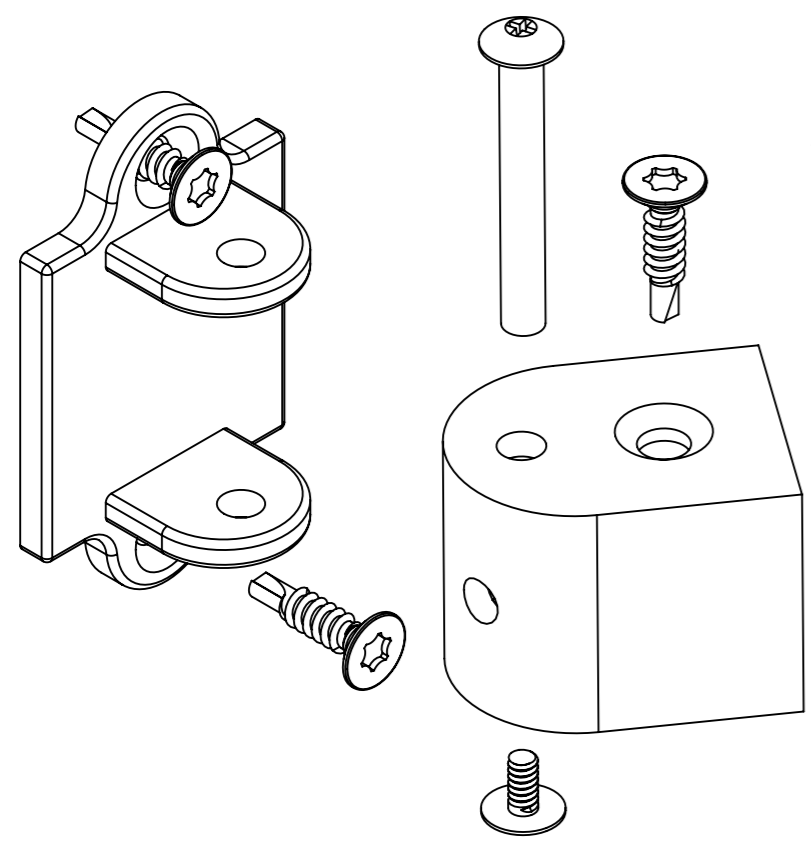
25mm Superior Horizontal Angle Bracket Supplied With Fixings & Used With Standard Panels & Posts
