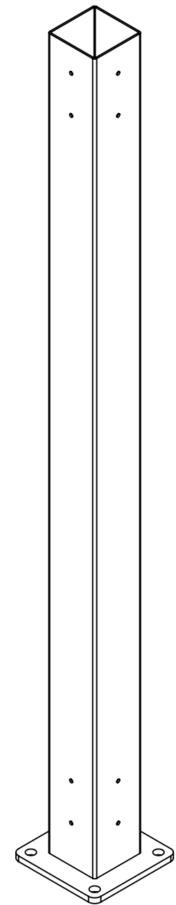
64PBC7511B CORNER POST 8 x Ø5 PILOT HOLES
