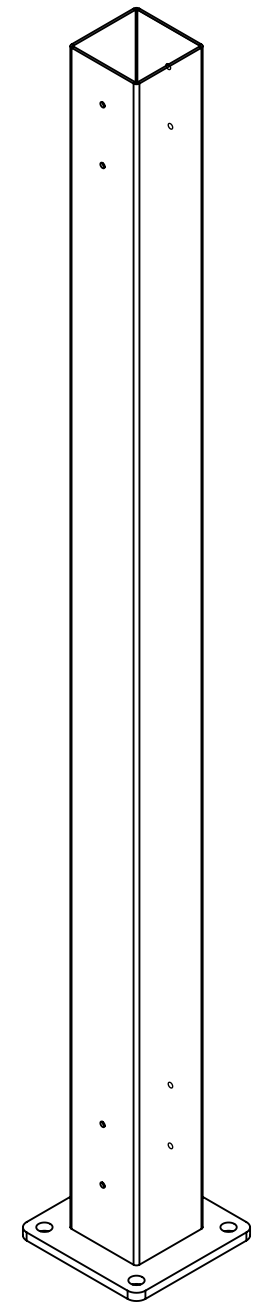
64PBM7511B MIDDLE POST 8 x Ø5 PILOT HOLES
