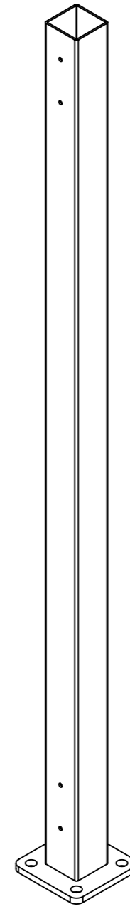
64PBE5011B END POST 4 x Ø5 PILOT HOLES
