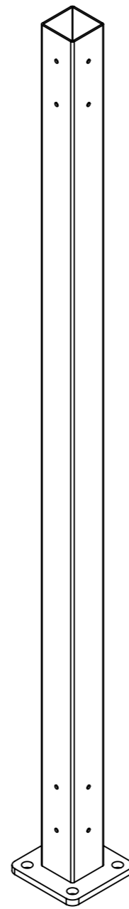
64PBC5011B CORNER POST 8 x Ø5 PILOT HOLES
