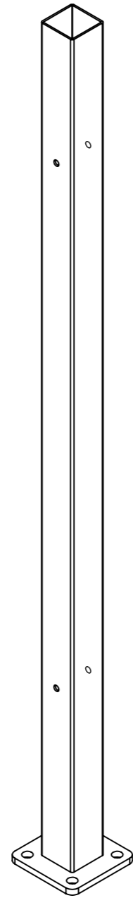
64PB76250B MIDDLE POST 4 x Ø8 PILOT HOLES
