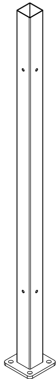
64PB76350B CORNER POST 4 x Ø8 PILOT HOLES
